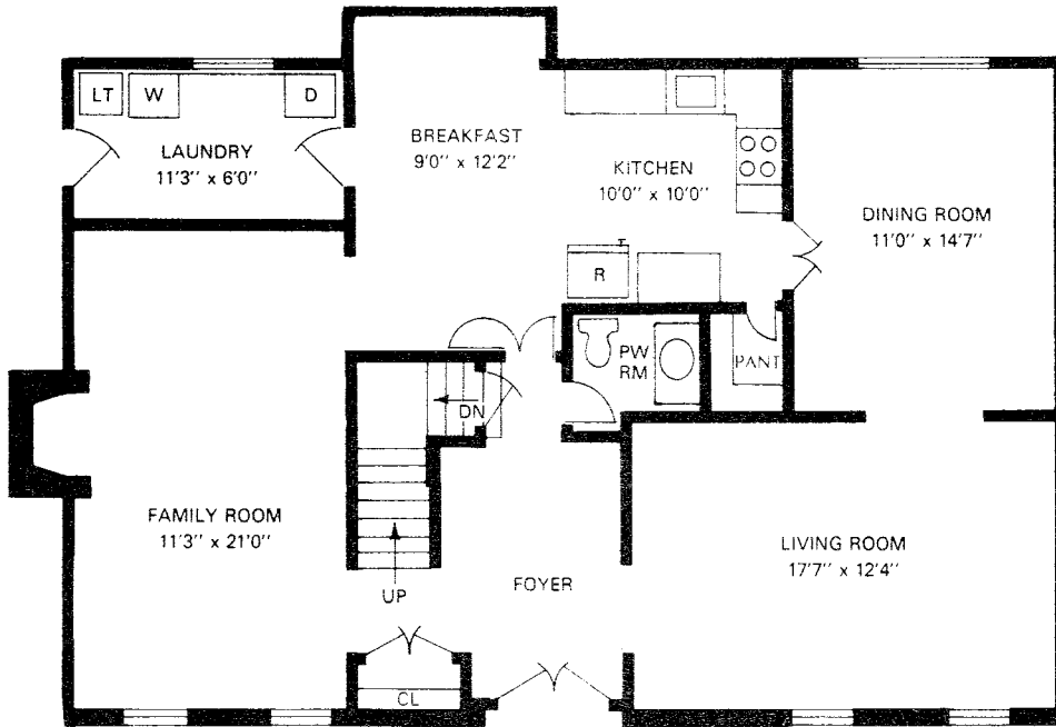
FIRST FLOOR FOXWOOD
