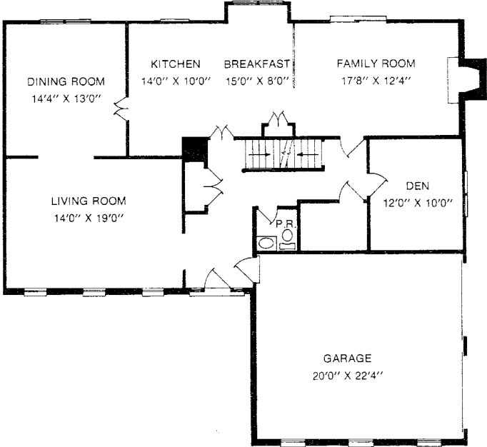
FIRST FLOOR WEDGEWOOD
